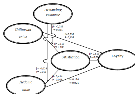
Figure 1: Line diagram of hypothesis testing result
